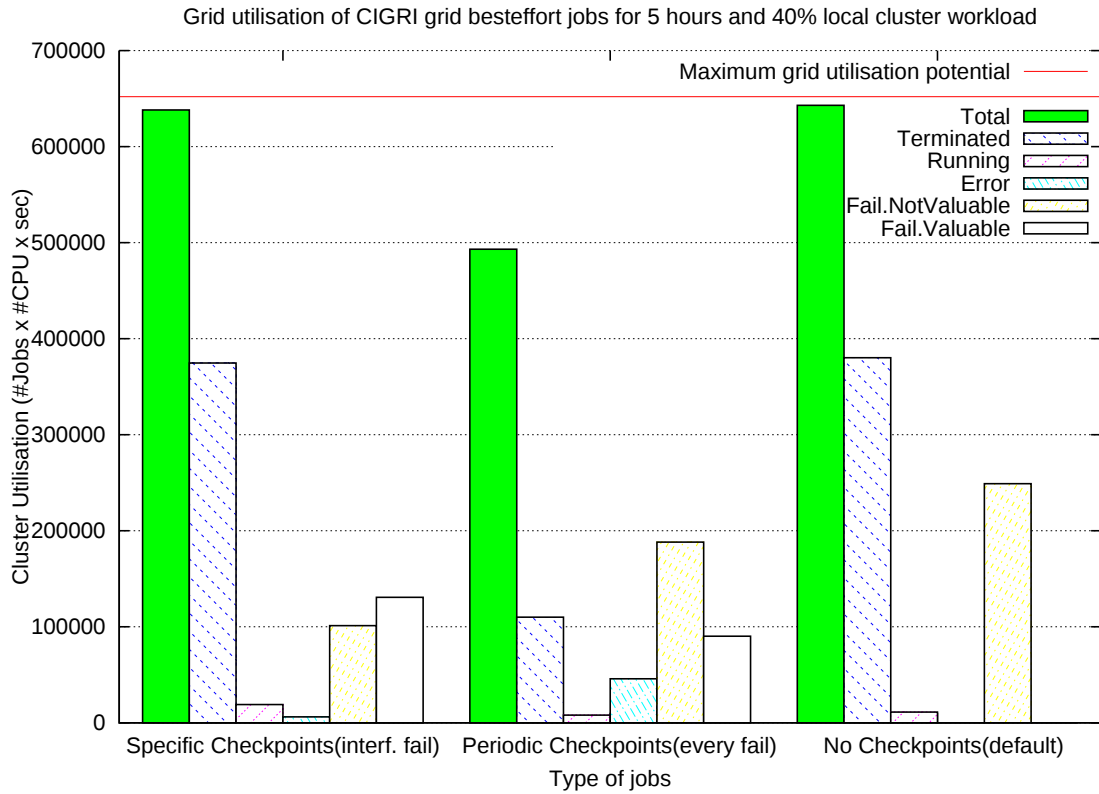
Figure 4.6: CIGRI grid utilization for 1 cluster of 32nodes grid (3 strategies comparison)
