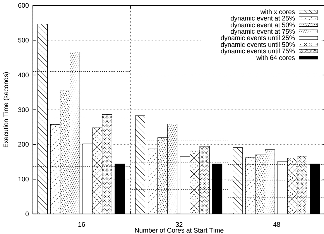
Figure 5.6: Growing in dynamic MPI application: execution time VS number of cores at starting time.
