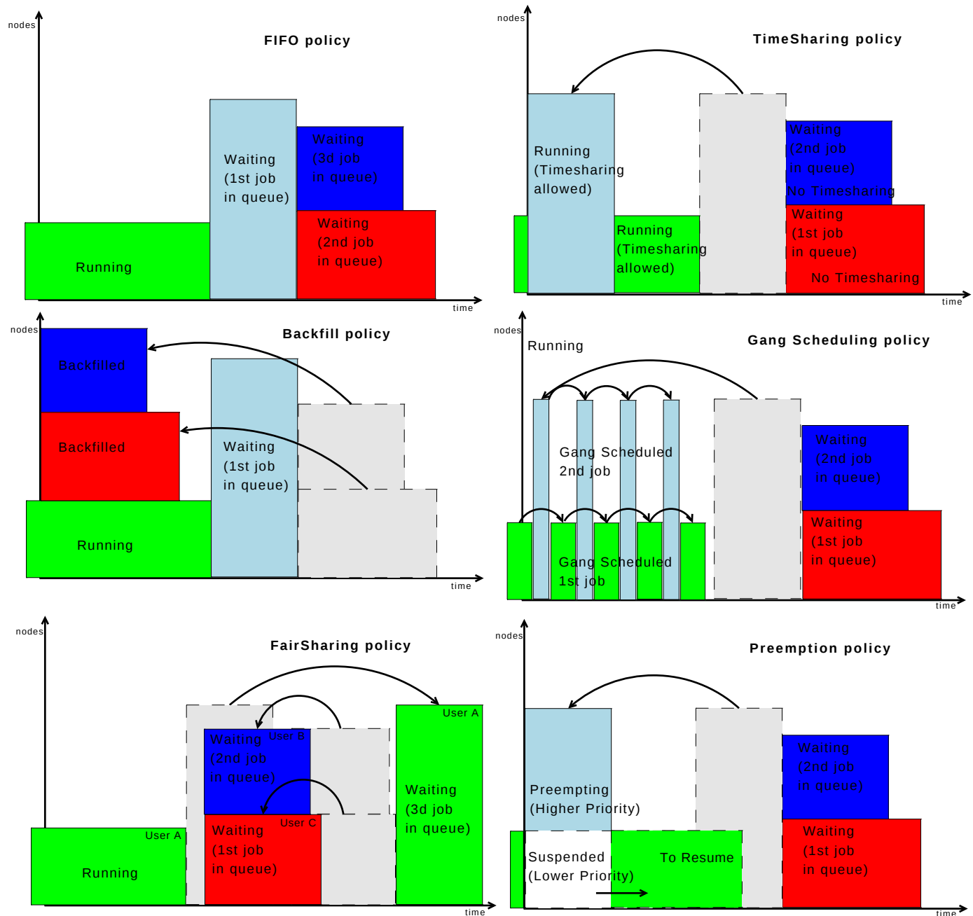
Figure 3.5: Function examples of Scheduling policies
